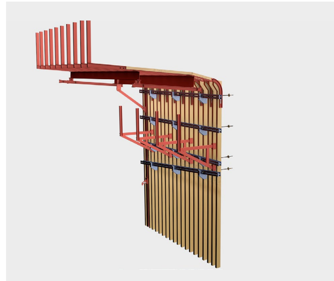
External formwork
