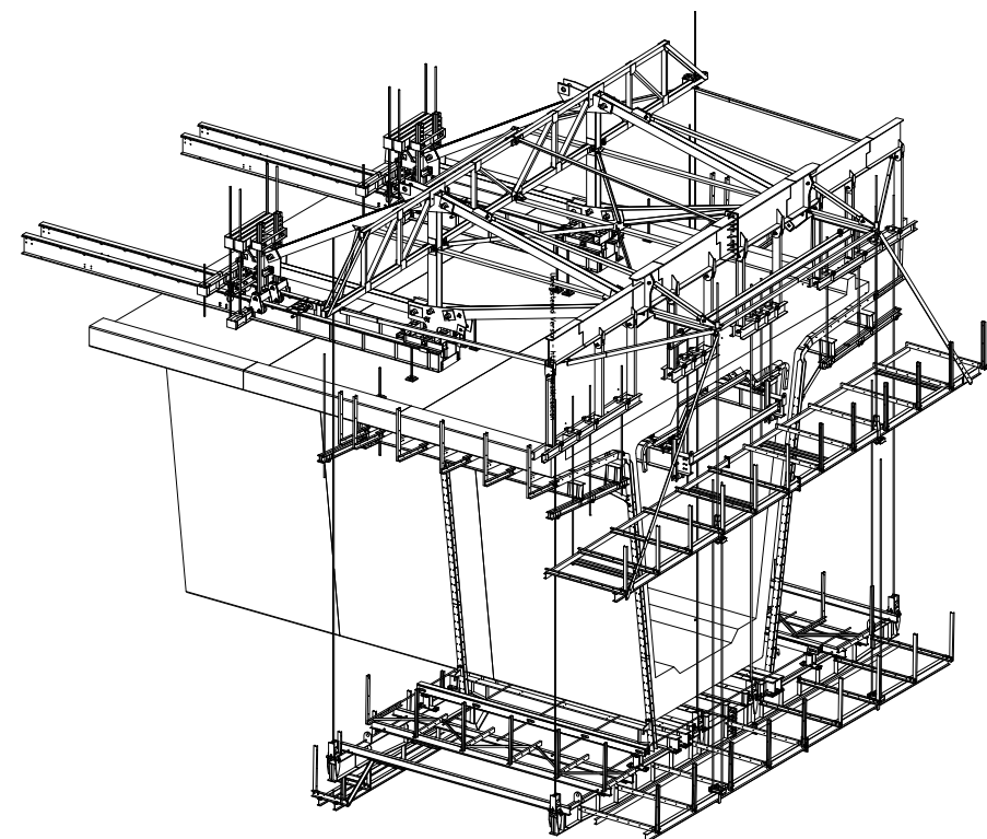
Overhead Form Traveller system
