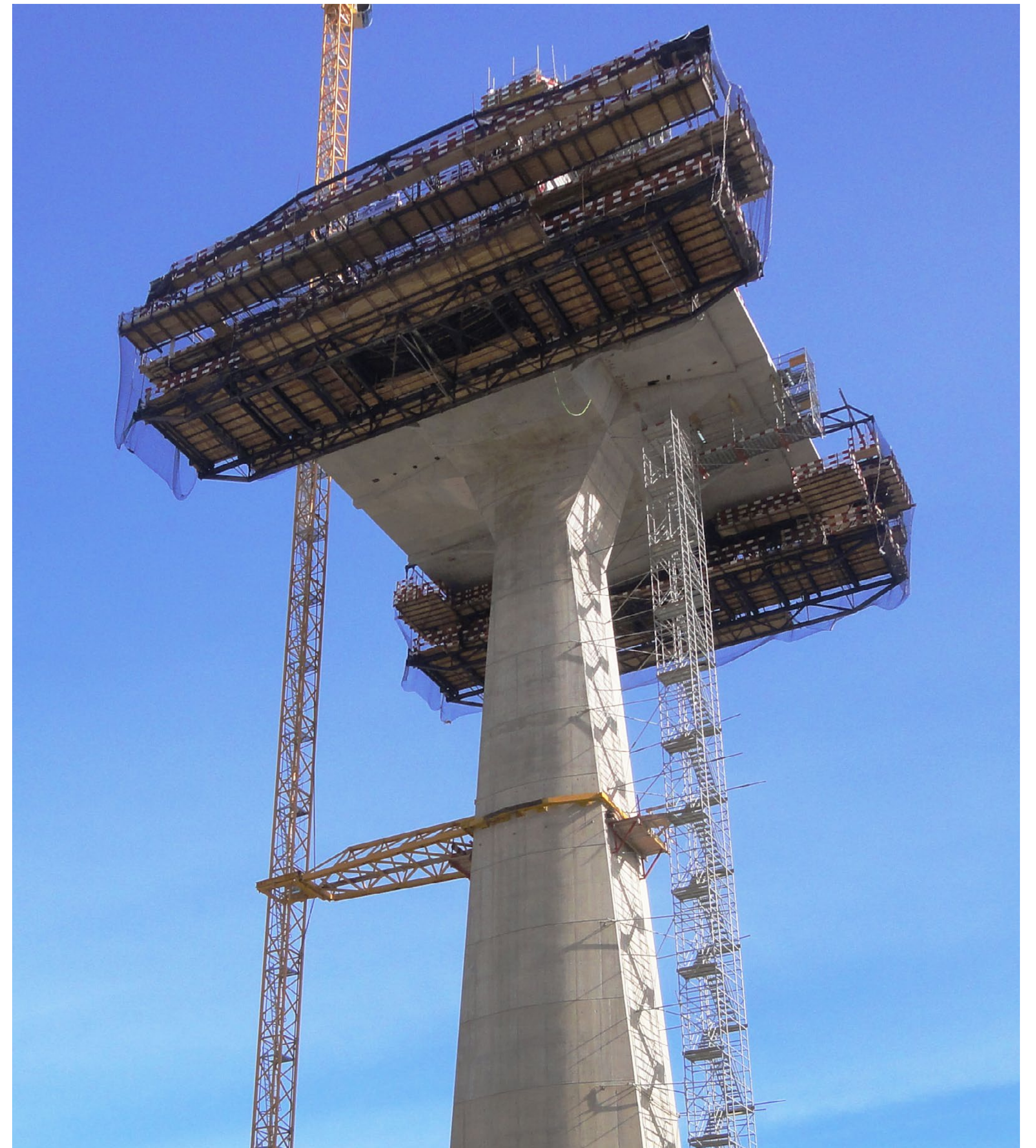
Overhead Form Traveller – Tua, Portugal
