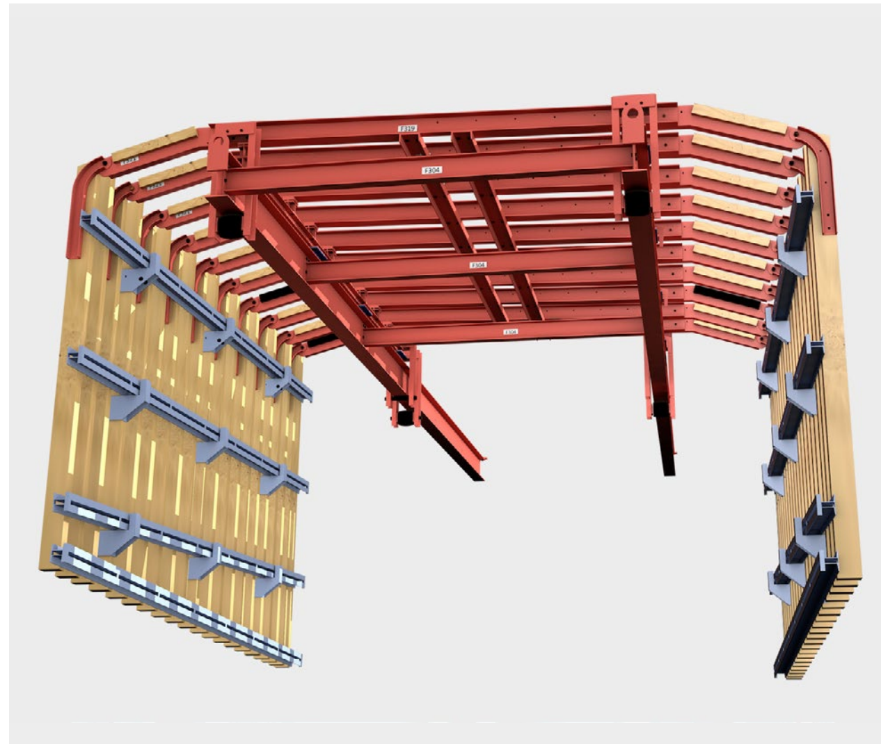
Internal formwork
